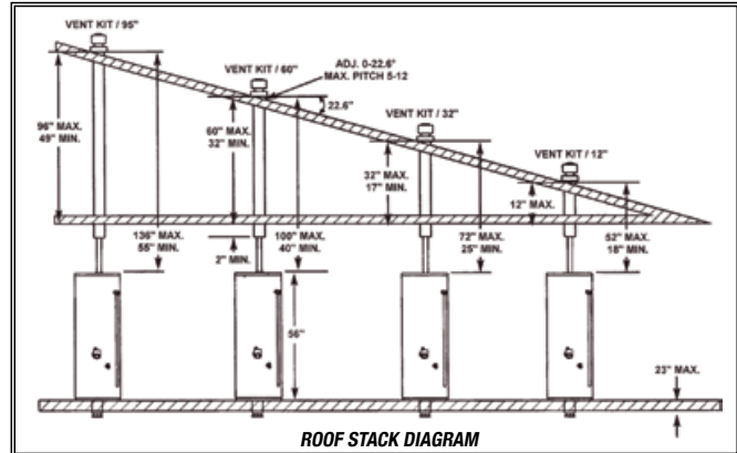
ROOF STACK DIAGRAM
